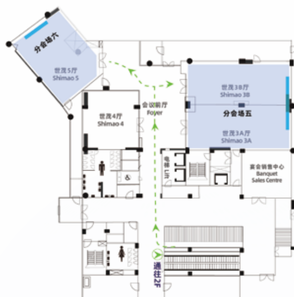
三楼裙楼会议室平面图 MEETING ROOM FLOOR PLAN ON LEVEL 3
